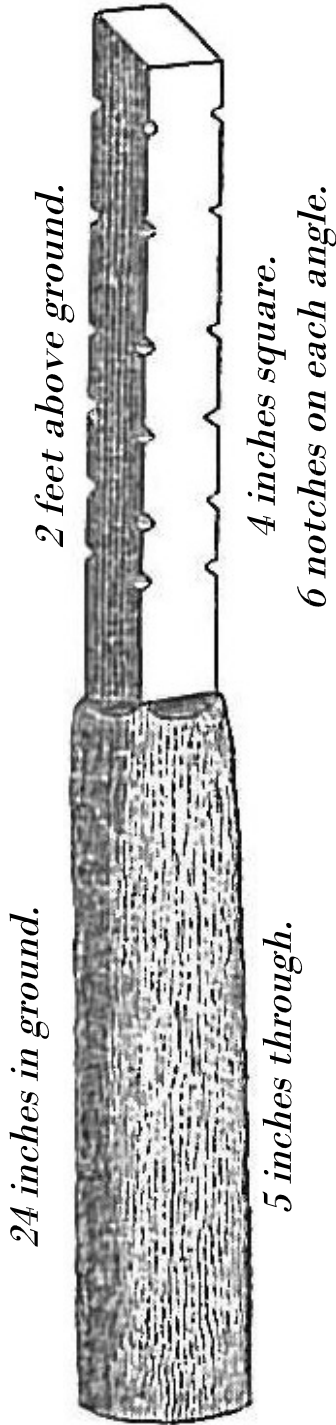
Township Corner Post Top bevelled, to turn rain.
